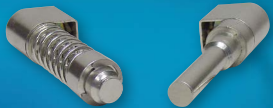
Silver-Nickel Contact Tip (85% Ag and 15% Ni)
