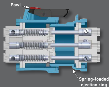
A spring-loaded ejection system ensures a quick break (15 ms) of the contacts.
